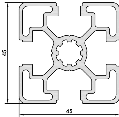
4456-2.3 AĞIRLIK / WEIGHT 1,545 kg/m
