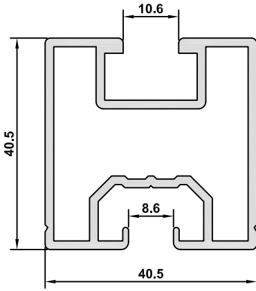
7666 AĞIRLIK / WEIGHT 1,008 kg/m
