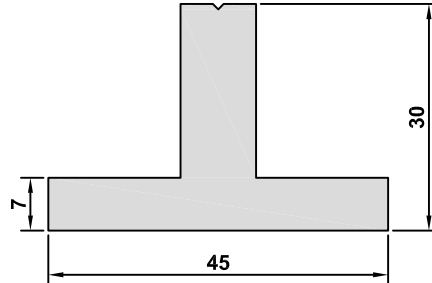
4485 AĞIRLIK / WEIGHT 1,477 kg/m
