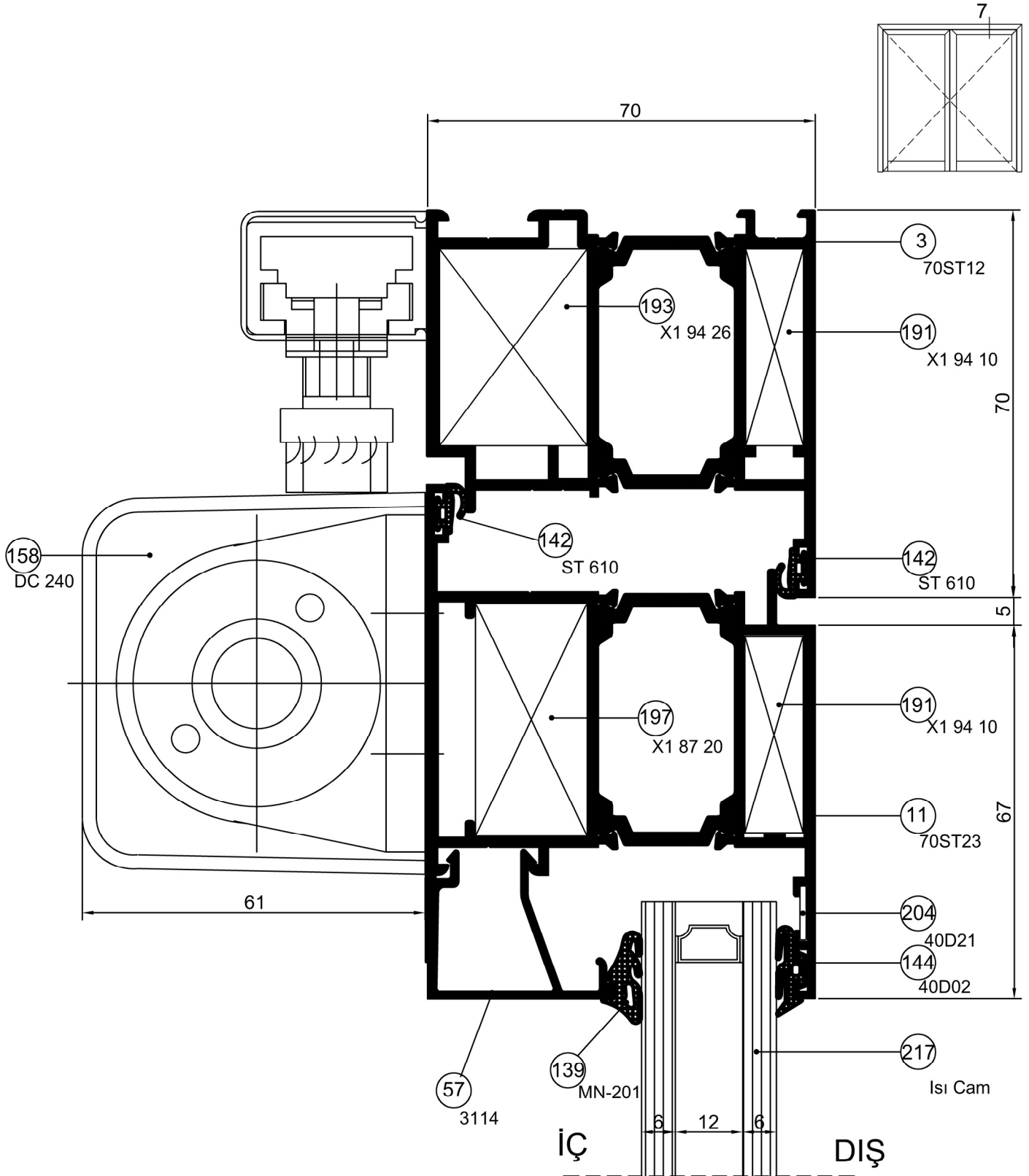
DETAIL ⑦ DETAYI
