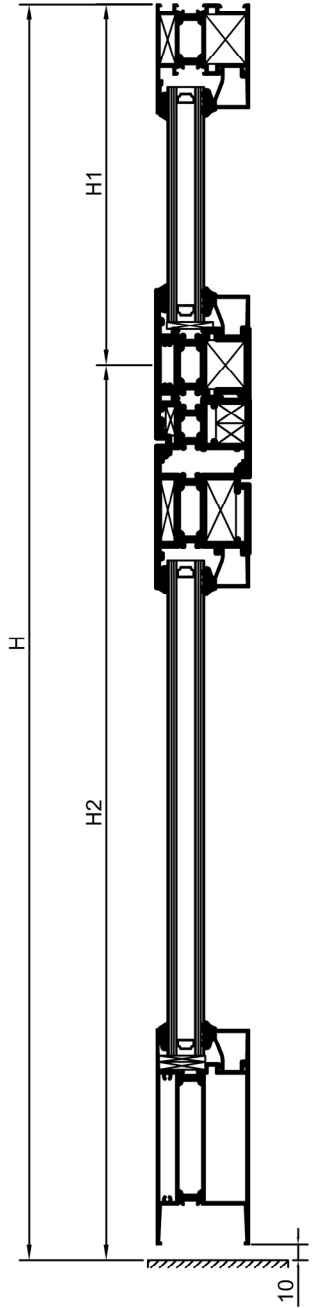
C-C Kesiti Section C-C
